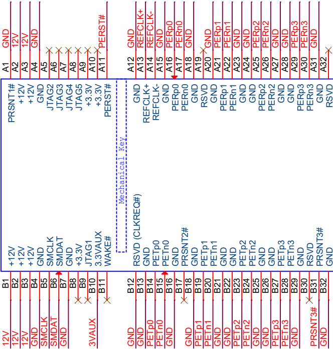
CN2 PCIe-X4-finger
